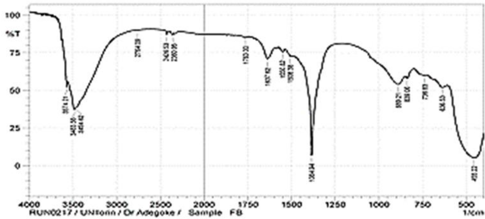
Figure 1: Fourier Transform Infrared (FTIR) transition spectrum of the synthesized ZnO-NP
