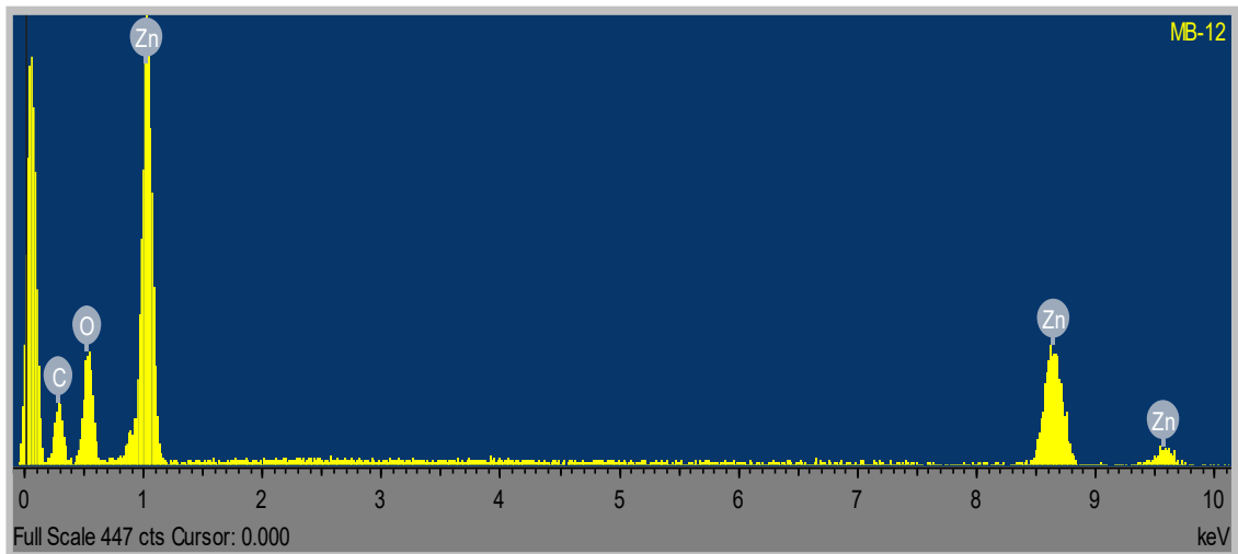
Figure 2: Energy diffraction X-Ray (EDX) of ZnO nanoparticle
