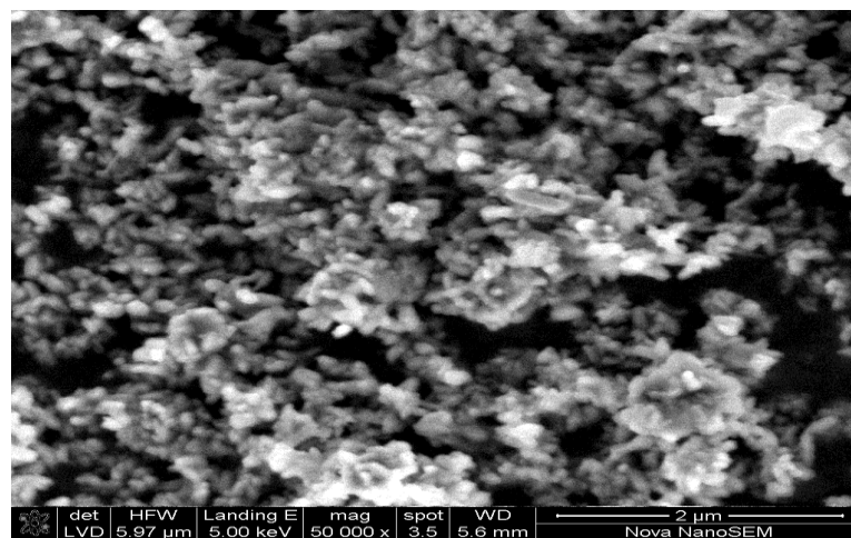
Figure 3: Scanning electron microscope (SEM) of the synthesized ZnO nanoparticle
